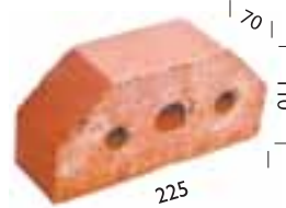
Double Cant
